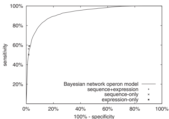
Fig. 3. ROC curve for our Bayes net operon model and operating points for the sequence-only, expression-only and sequence+expression models.
