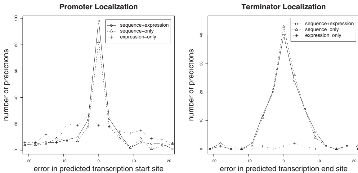
Fig. 2. Histograms of errors in predicted transcription start positions and predicted transcription termination positions. Histograms are shown for all three models considered in the experiments.
